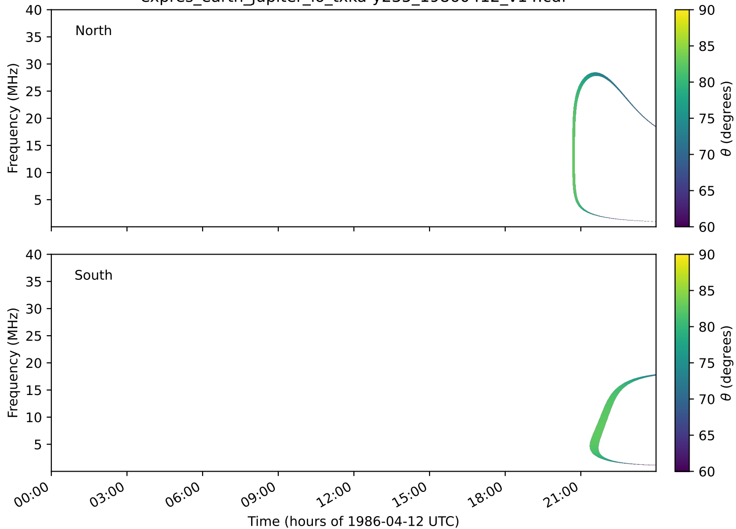
expres_earth_jupiter_io_txka-y235_19860412_v14.cdf
