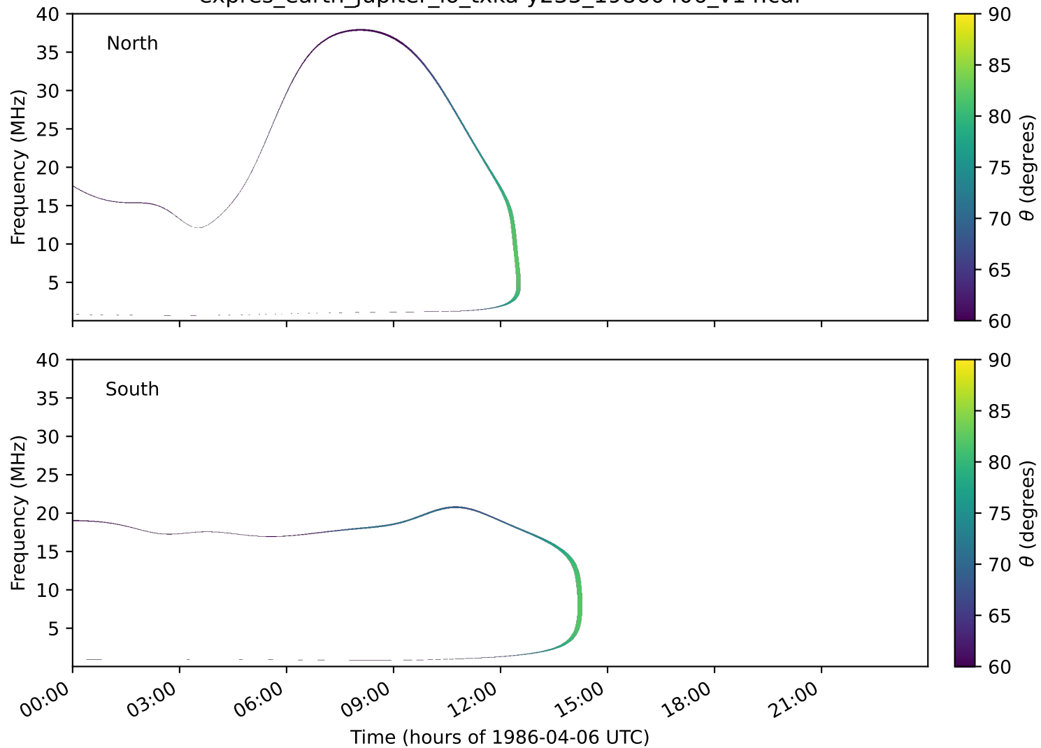
expres_earth_jupiter_io_txka-y235_19860406_v14.cdf
