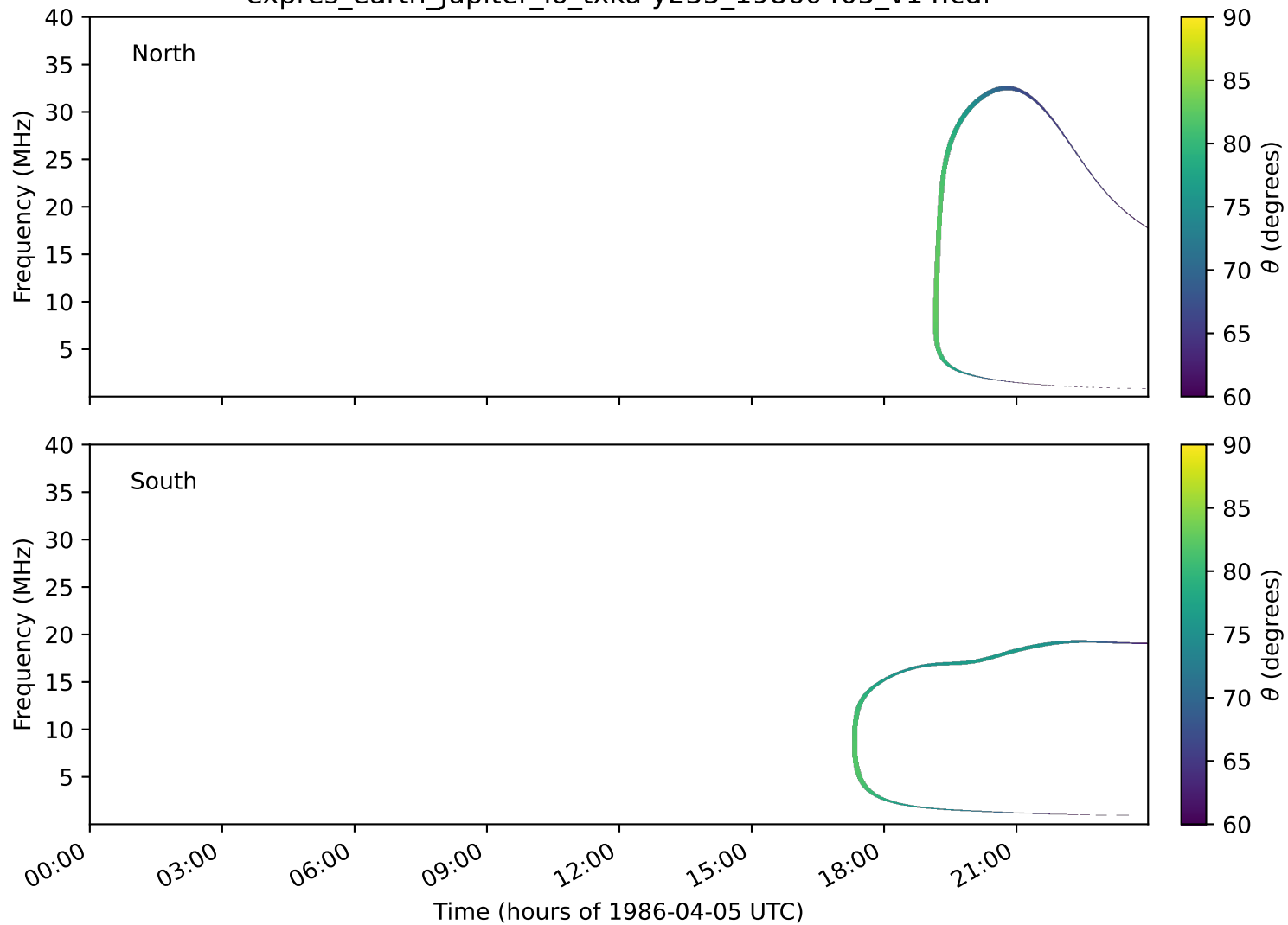
expres_earth_jupiter_io_txka-y235_19860405_v14.cdf
