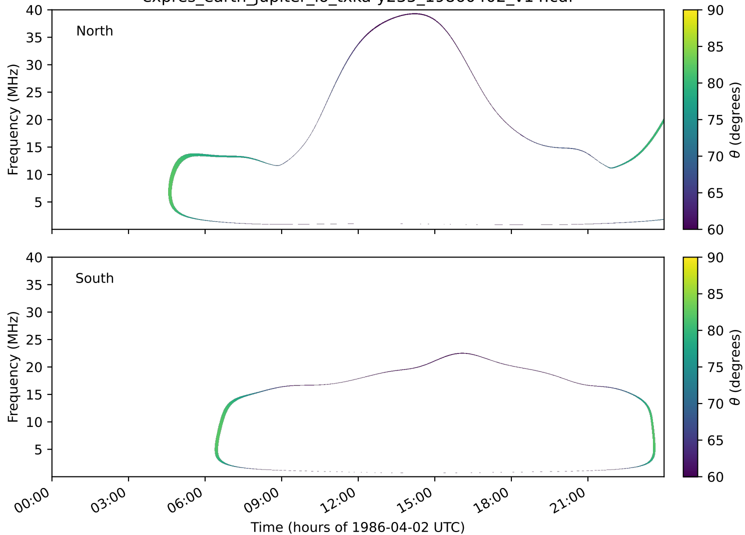
expres_earth_jupiter_io_txka-y235_19860402_v14.cdf
