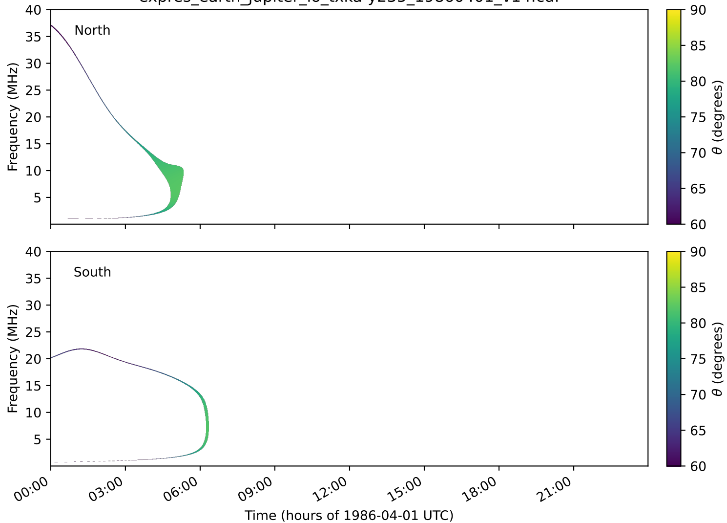
expres_earth_jupiter_io_txka-y235_19860401_v14.cdf
