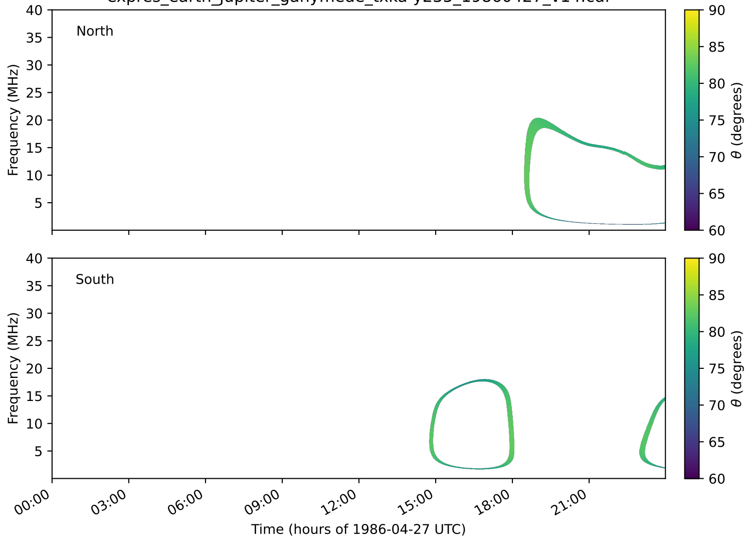
expres_earth_jupiter_ganymede_txka-y235_19860427_v14.cdf
