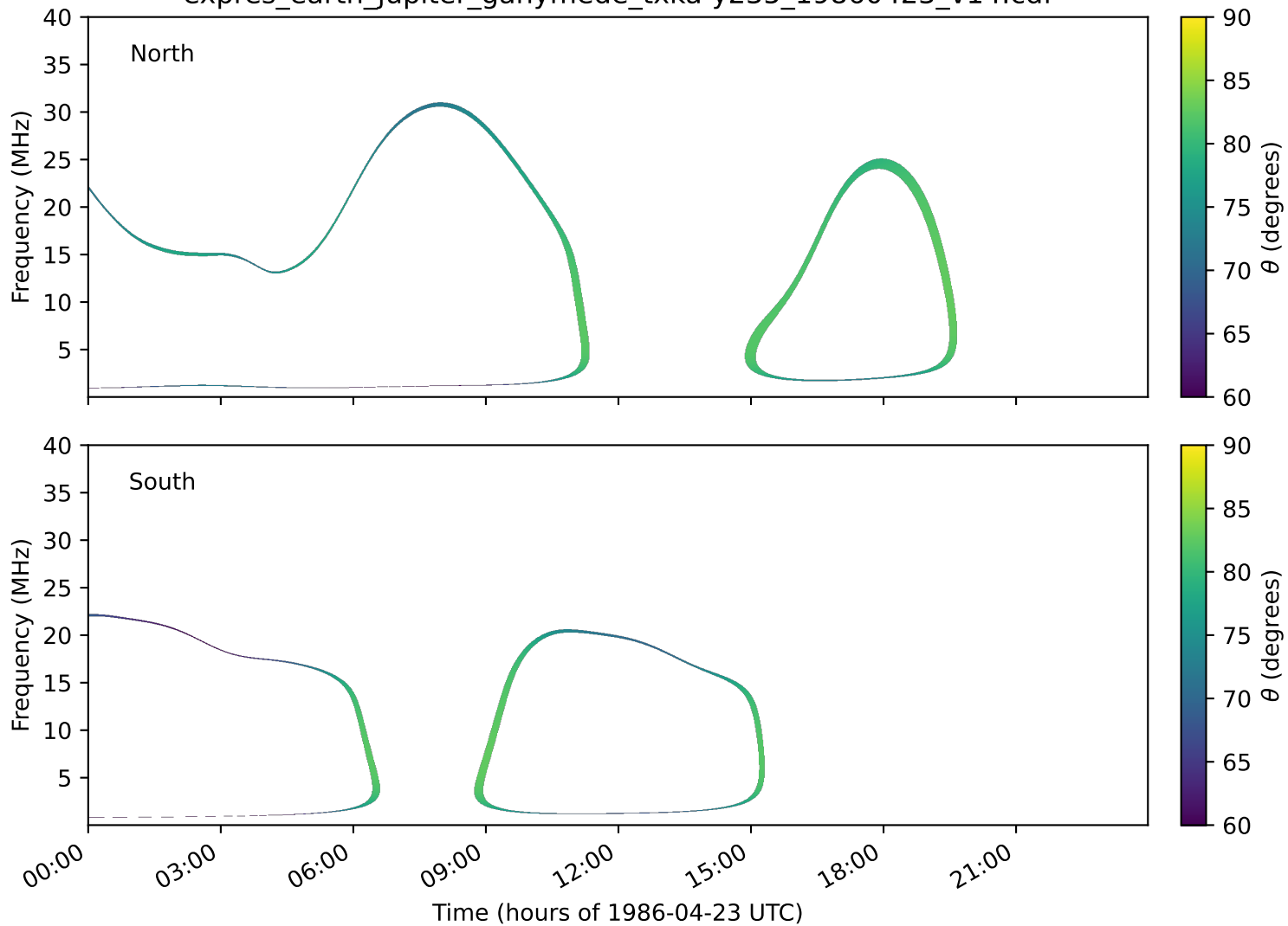
expres_earth_jupiter_ganymede_txka-y235_19860423_v14.cdf
