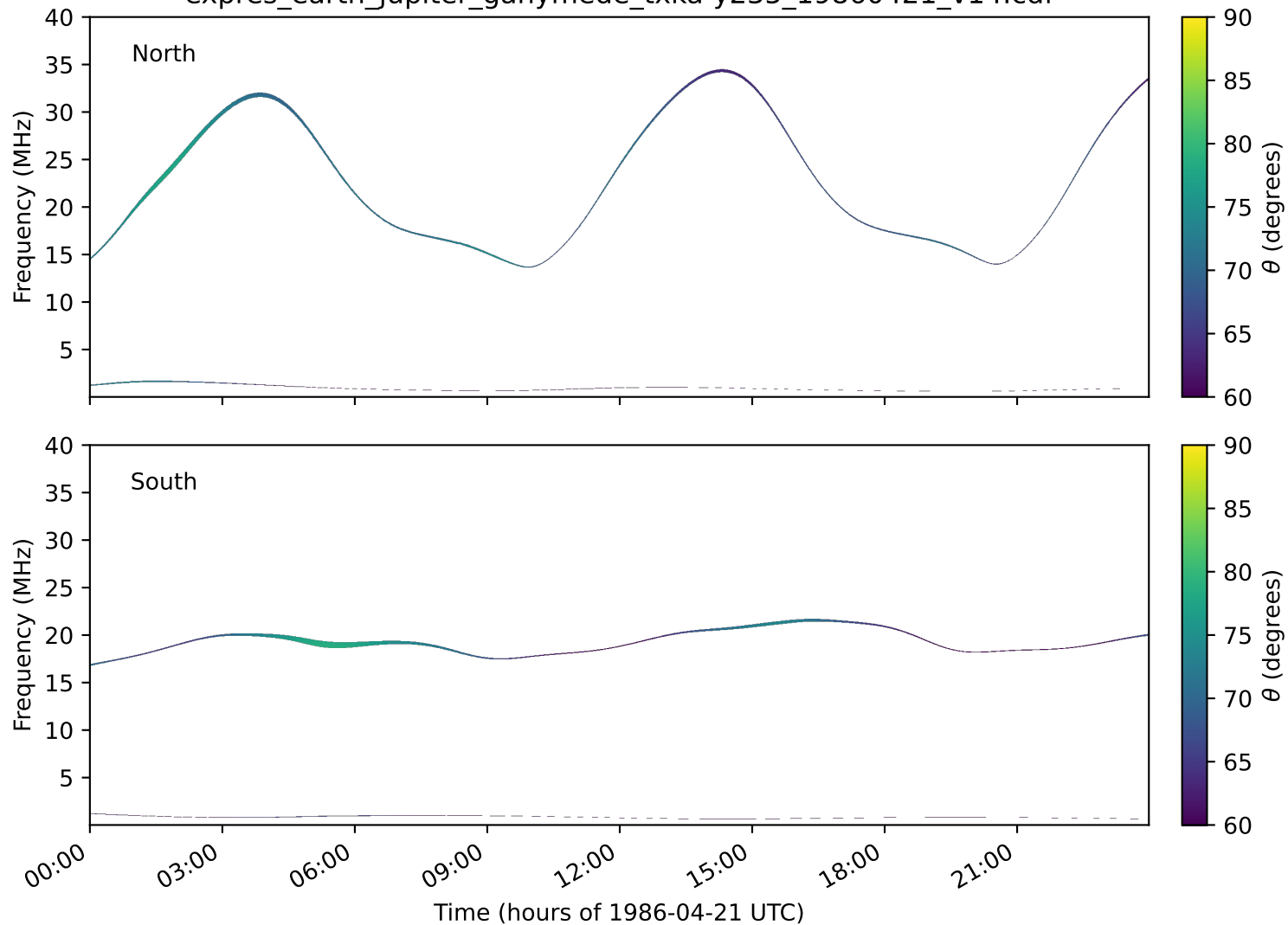
expres_earth_jupiter_ganymede_txka-y235_19860421_v14.cdf
