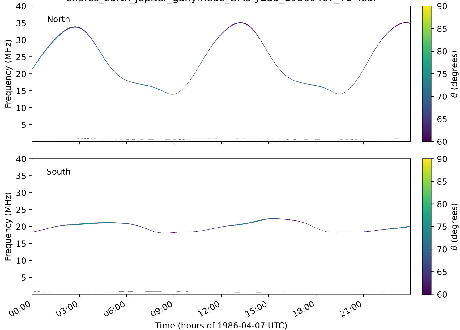
expres_earth_jupiter_ganymede_txka-y235_19860407_v14.cdf
