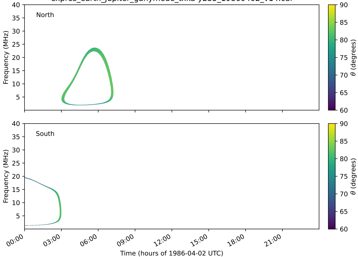
expres_earth_jupiter_ganymede_txka-y235_19860402_v14.cdf
