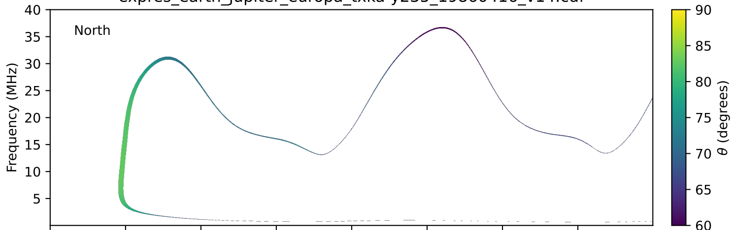
expres_earth_jupiter_europa_txka-y235_19860416_v14.cdf
