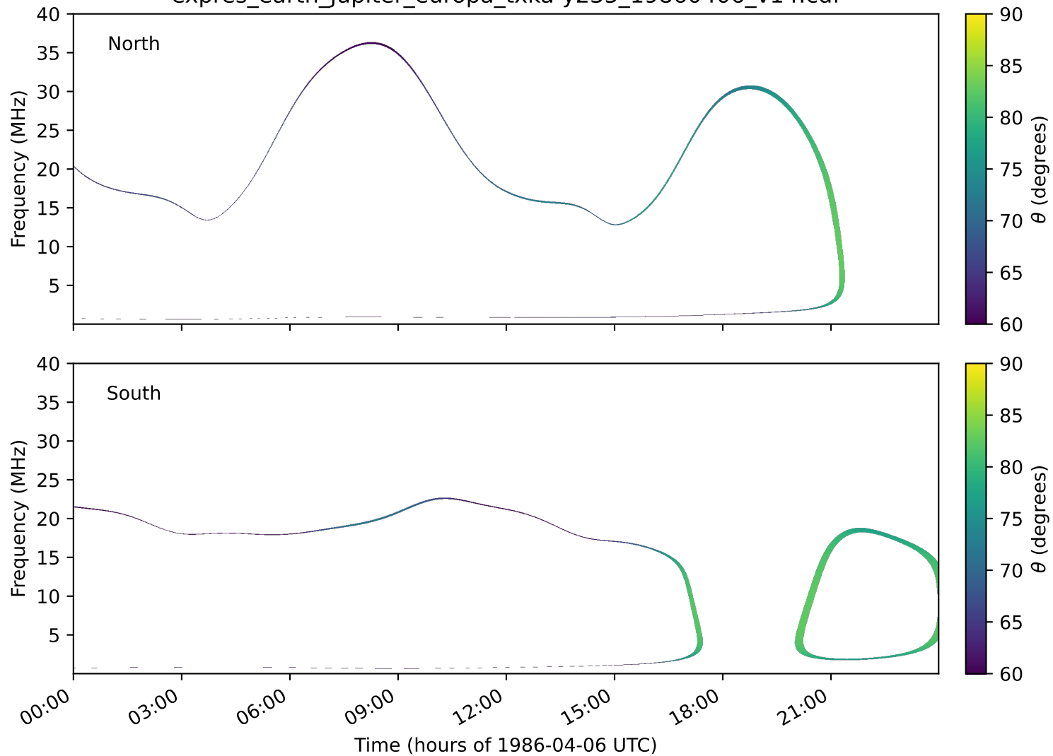
expres_earth_jupiter_europa_txka-y235_19860406_v14.cdf
