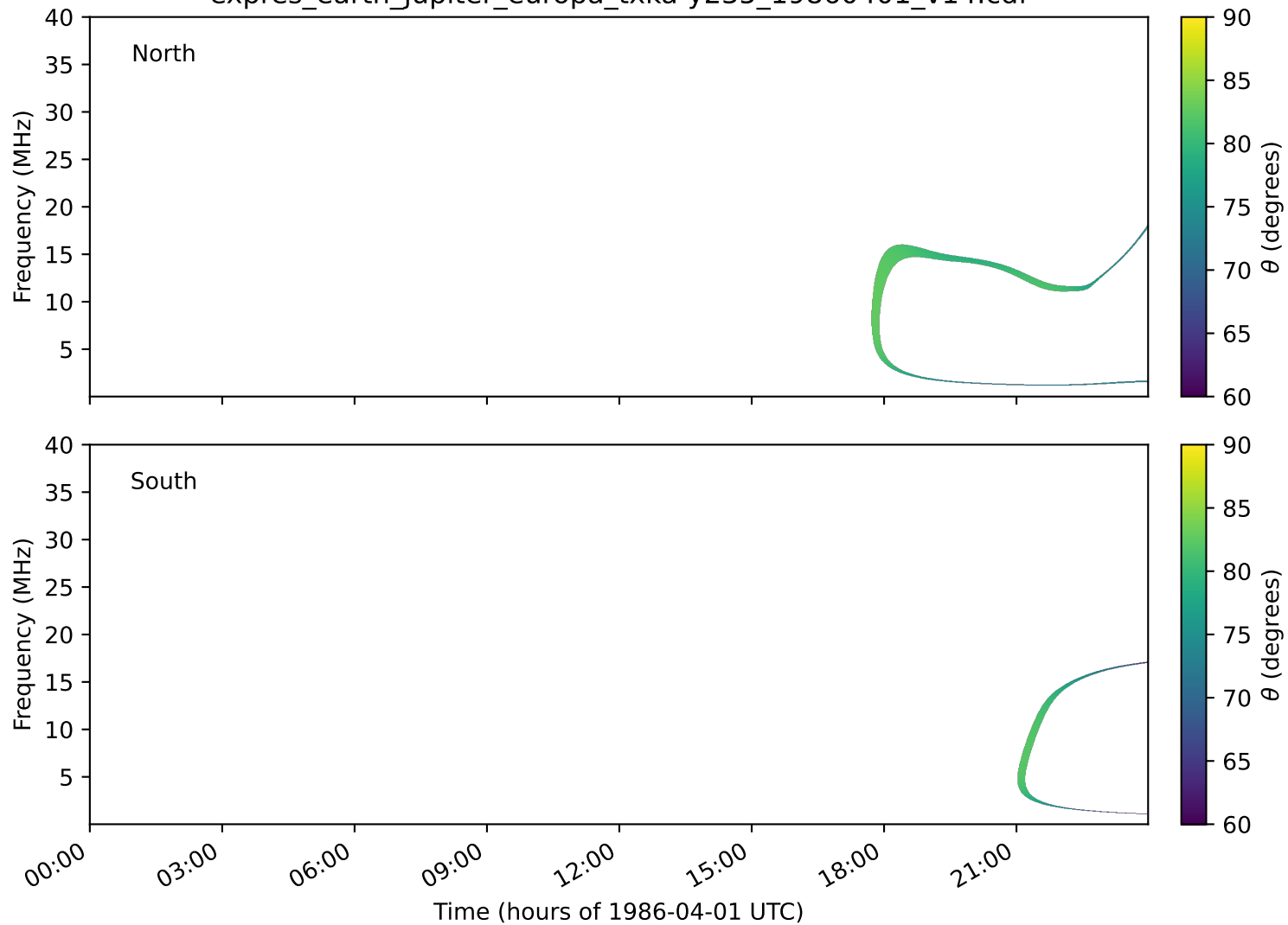
expres_earth_jupiter_europa_txka-y235_19860401_v14.cdf
