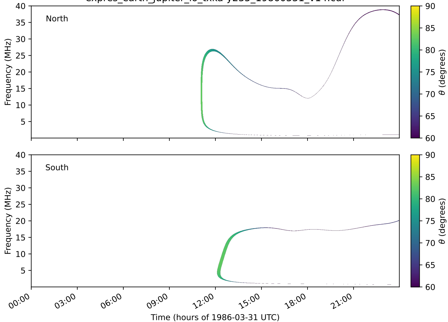
expres_earth_jupiter_io_txka-y235_19860331_v14.cdf
