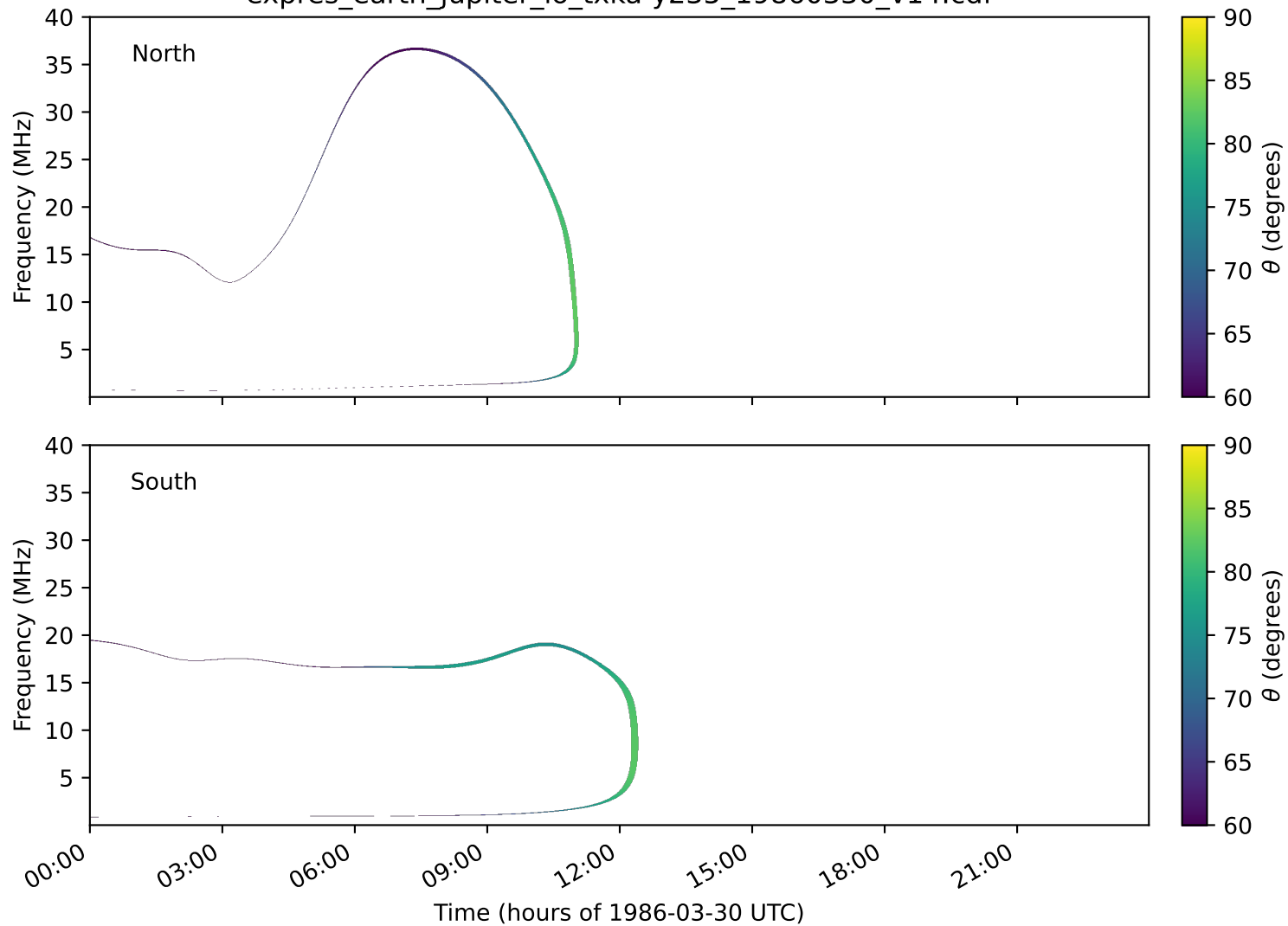
expres_earth_jupiter_io_txka-y235_19860330_v14.cdf
