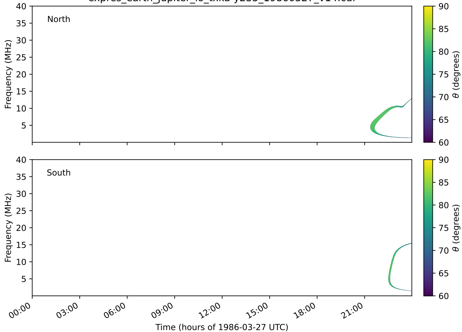
expres_earth_jupiter_io_txka-y235_19860327_v14.cdf
