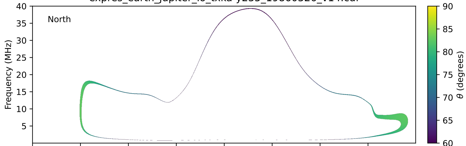
expres_earth_jupiter_io_txka-y235_19860326_v14.cdf
