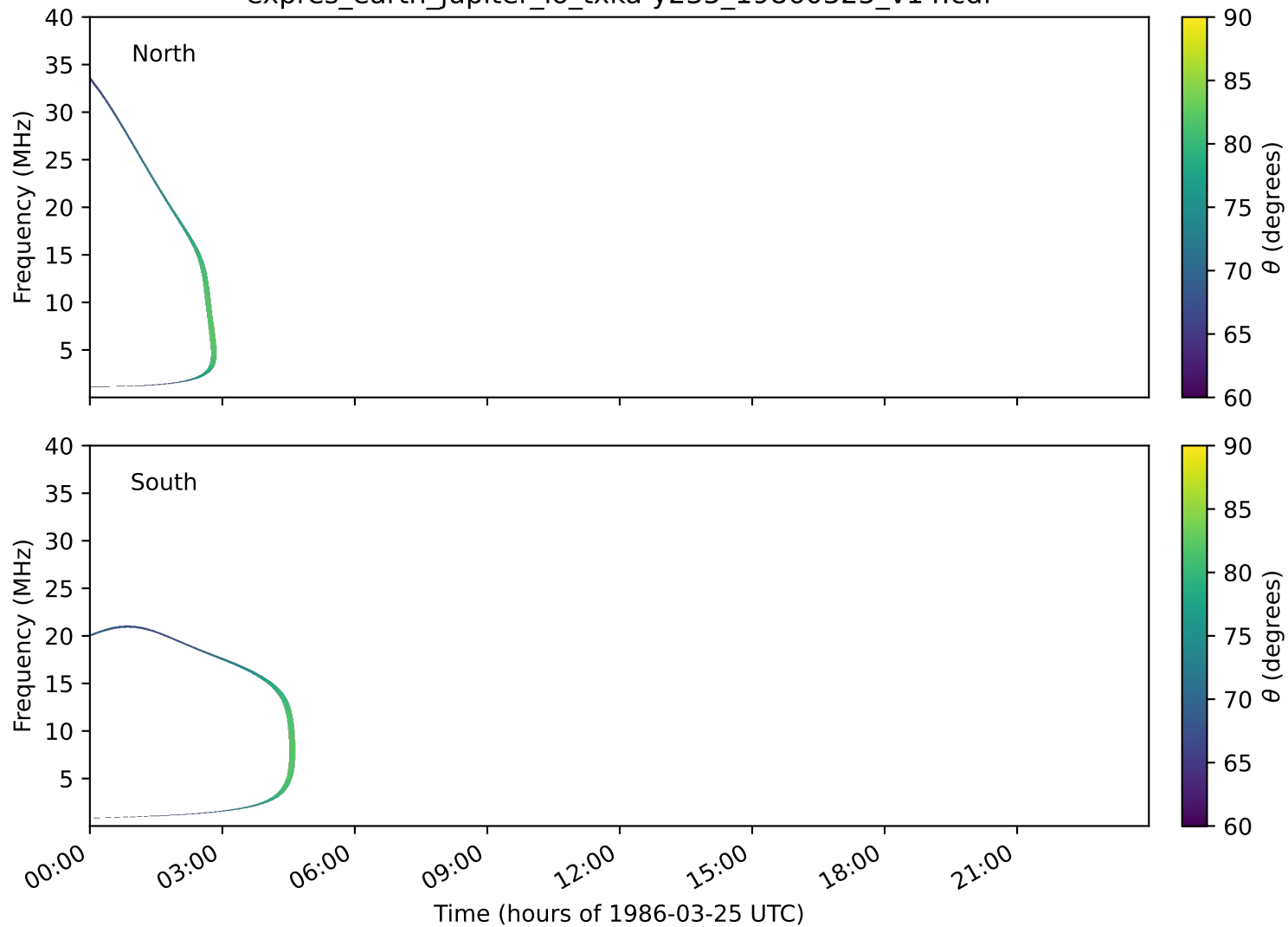
expres_earth_jupiter_io_txka-y235_19860325_v14.cdf
