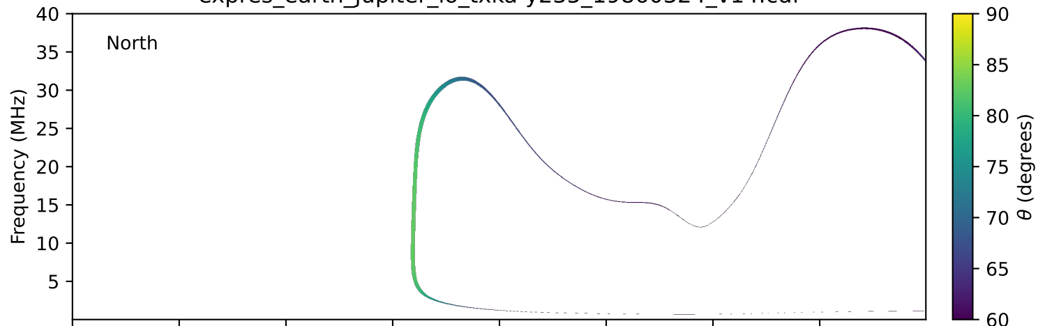
expres_earth_jupiter_io_txka-y235_19860324_v14.cdf
