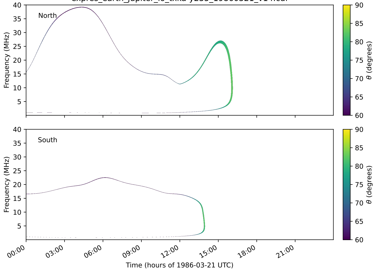
expres_earth_jupiter_io_txka-y235_19860321_v14.cdf
