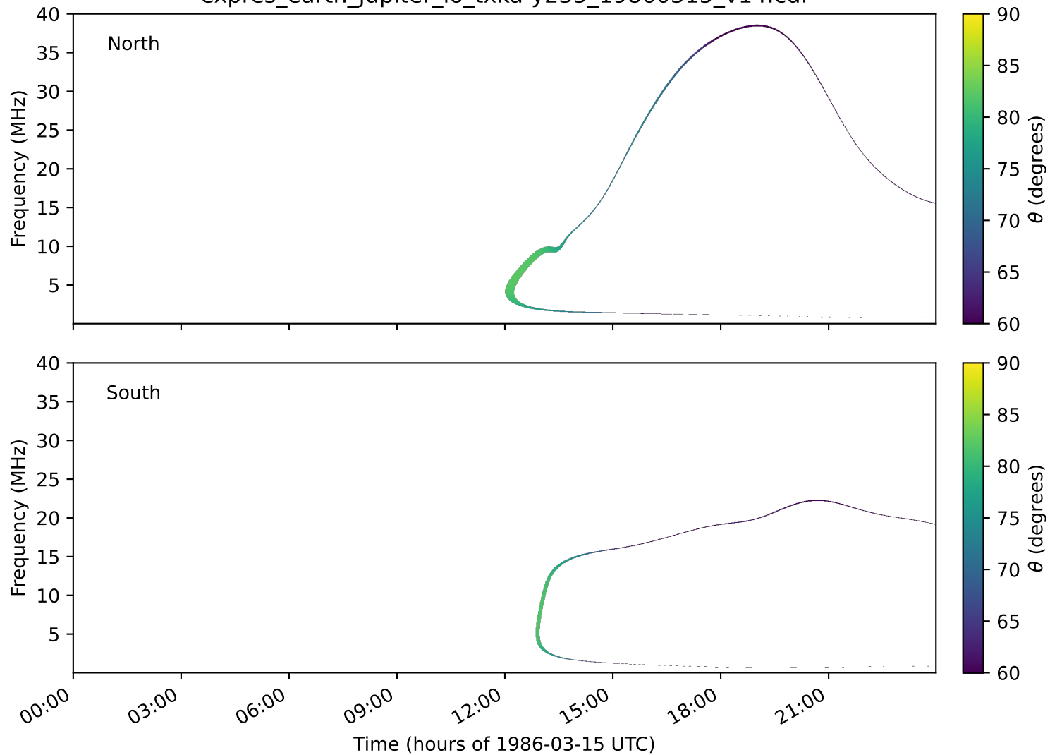
expres_earth_jupiter_io_txka-y235_19860315_v14.cdf
