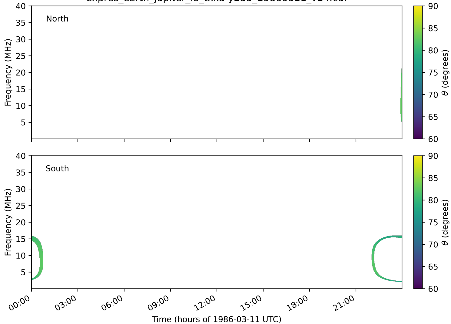
expres_earth_jupiter_io_txka-y235_19860311_v14.cdf
