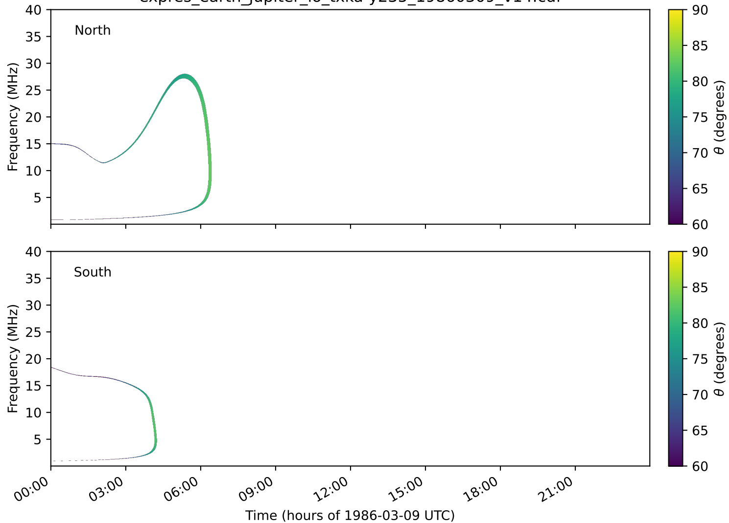
expres_earth_jupiter_io_txka-y235_19860309_v14.cdf
