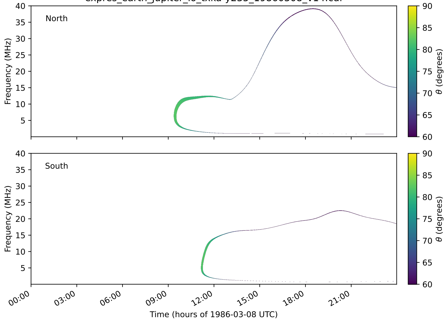
expres_earth_jupiter_io_txka-y235_19860308_v14.cdf
