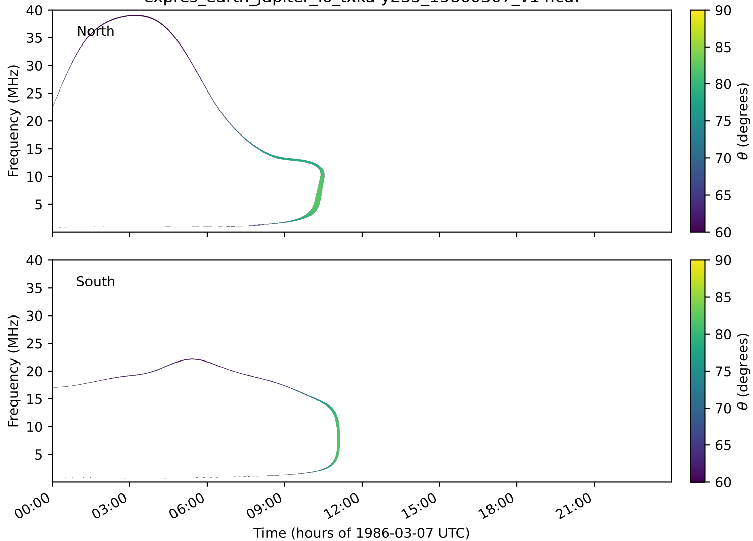
expres_earth_jupiter_io_txka-y235_19860307_v14.cdf
