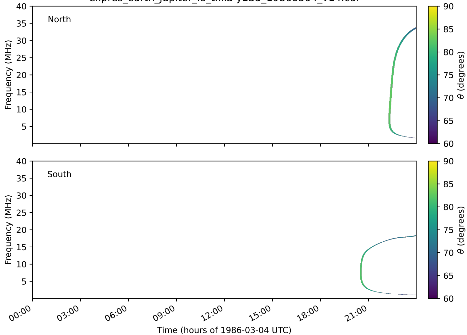
expres_earth_jupiter_io_txka-y235_19860304_v14.cdf
