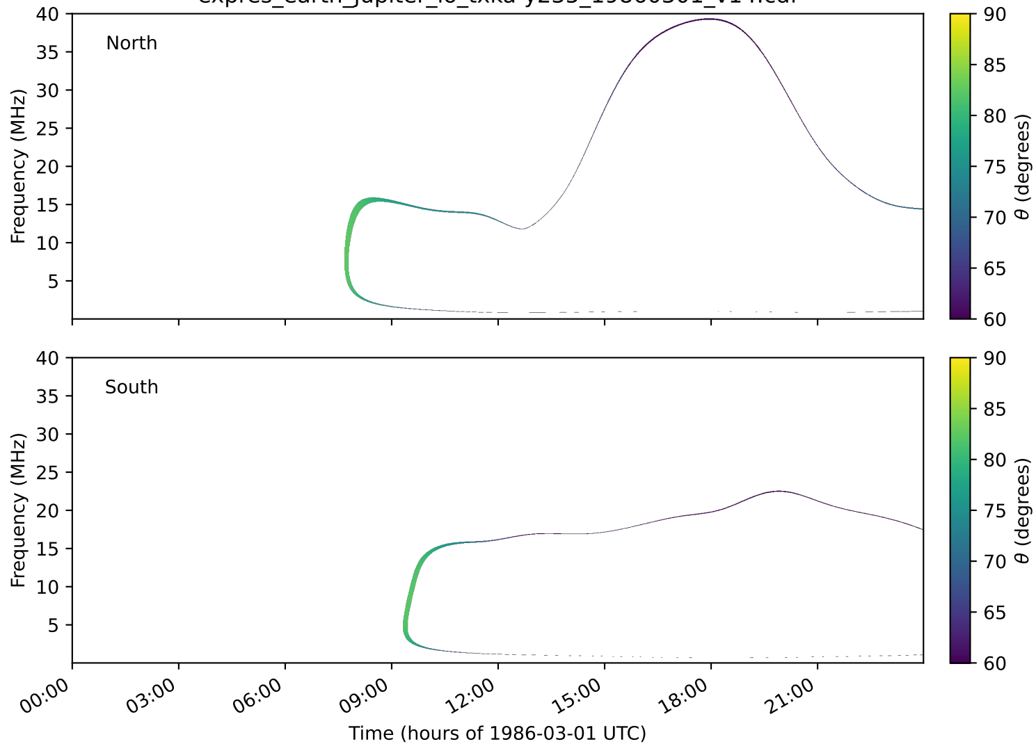
expres_earth_jupiter_io_txka-y235_19860301_v14.cdf
