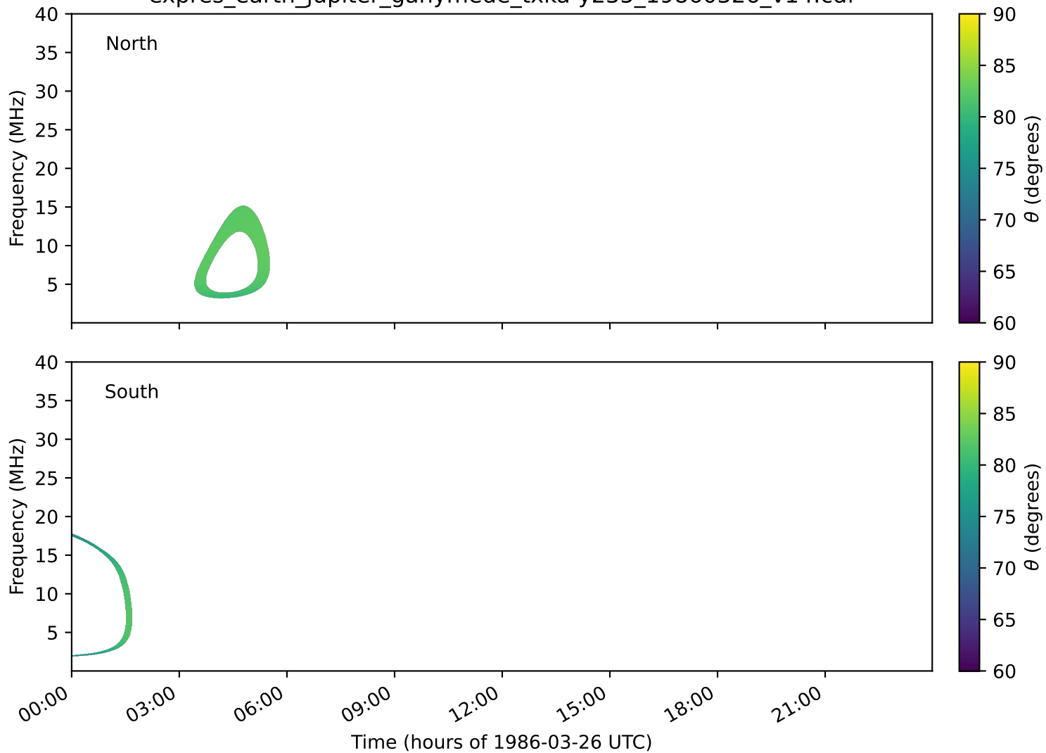
expres_earth_jupiter_ganymede_txka-y235_19860326_v14.cdf
