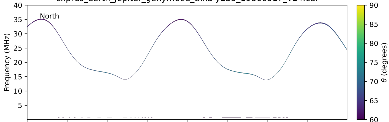
expres_earth_jupiter_ganymede_txka-y235_19860317_v14.cdf
