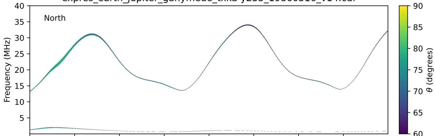
expres_earth_jupiter_ganymede_txka-y235_19860316_v14.cdf
