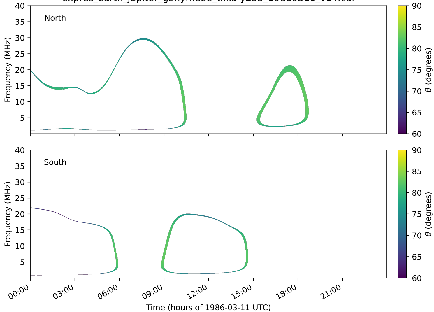
expres_earth_jupiter_ganymede_txka-y235_19860311_v14.cdf
