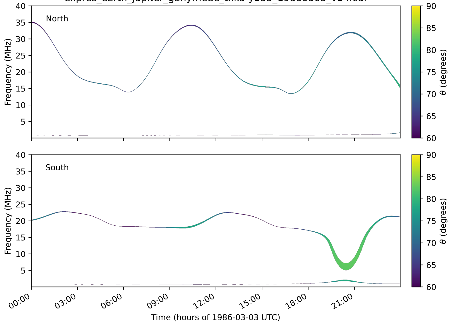
expres_earth_jupiter_ganymede_txka-y235_19860303_v14.cdf
