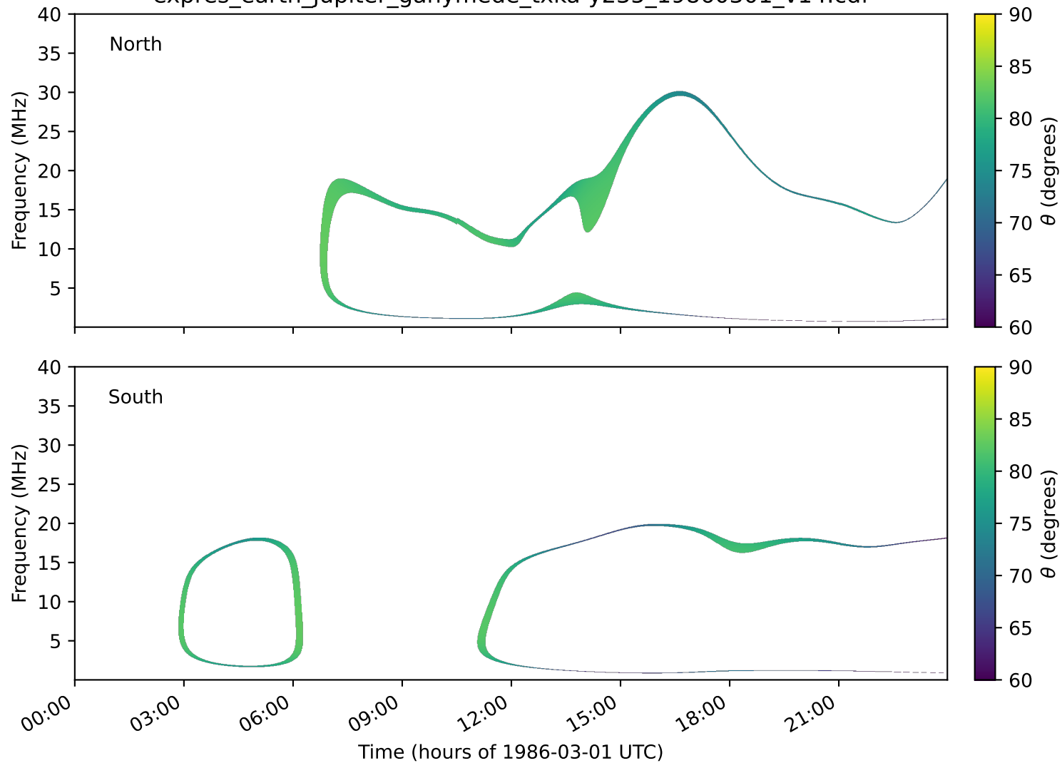
expres_earth_jupiter_ganymede_txka-y235_19860301_v14.cdf
