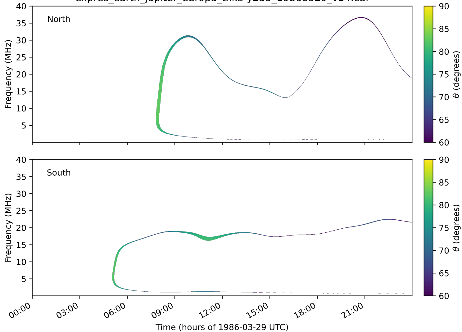
expres_earth_jupiter_europa_txka-y235_19860329_v14.cdf
