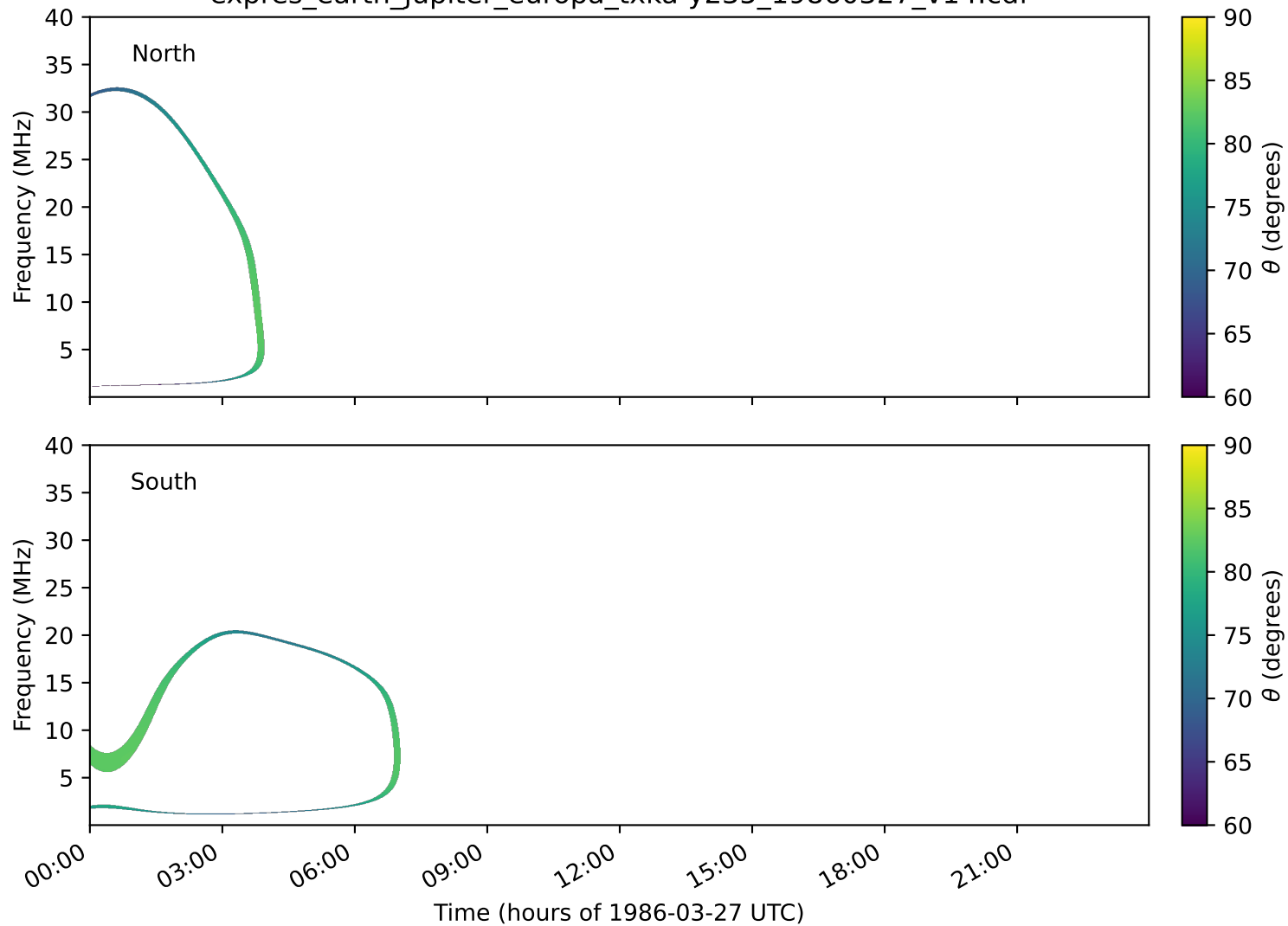
expres_earth_jupiter_europa_txka-y235_19860327_v14.cdf
