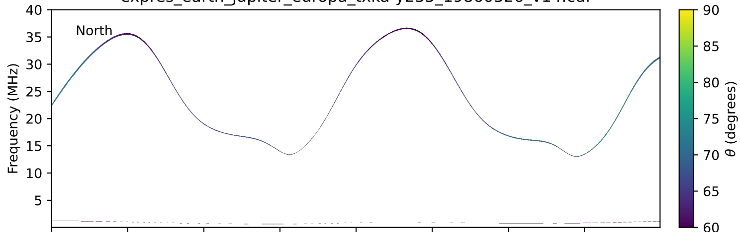
expres_earth_jupiter_europa_txka-y235_19860326_v14.cdf
