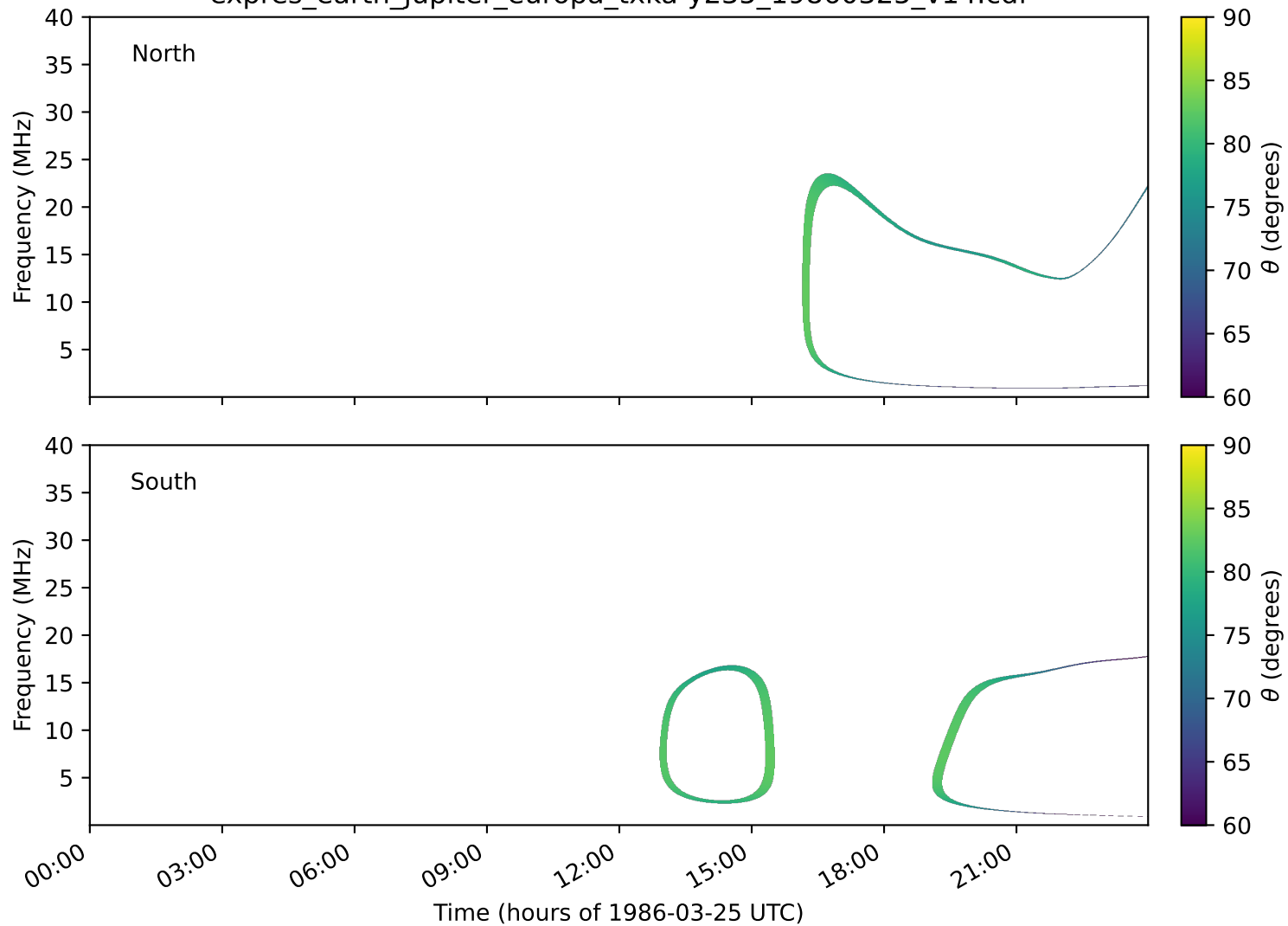
expres_earth_jupiter_europa_txka-y235_19860325_v14.cdf
