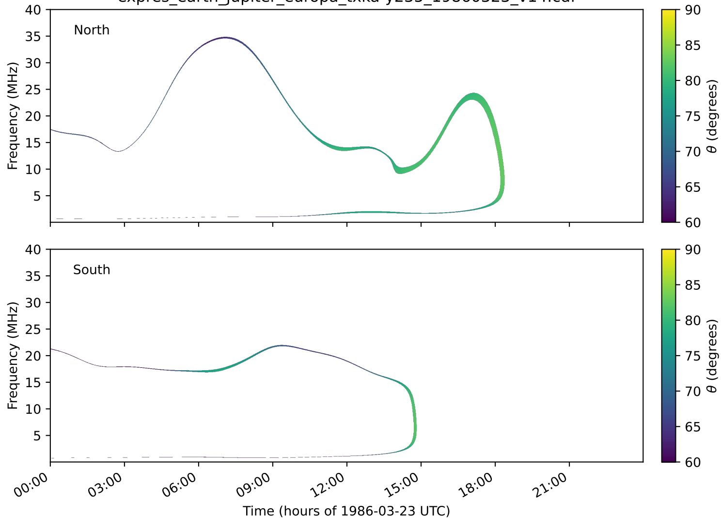
expres_earth_jupiter_europa_txka-y235_19860323_v14.cdf
