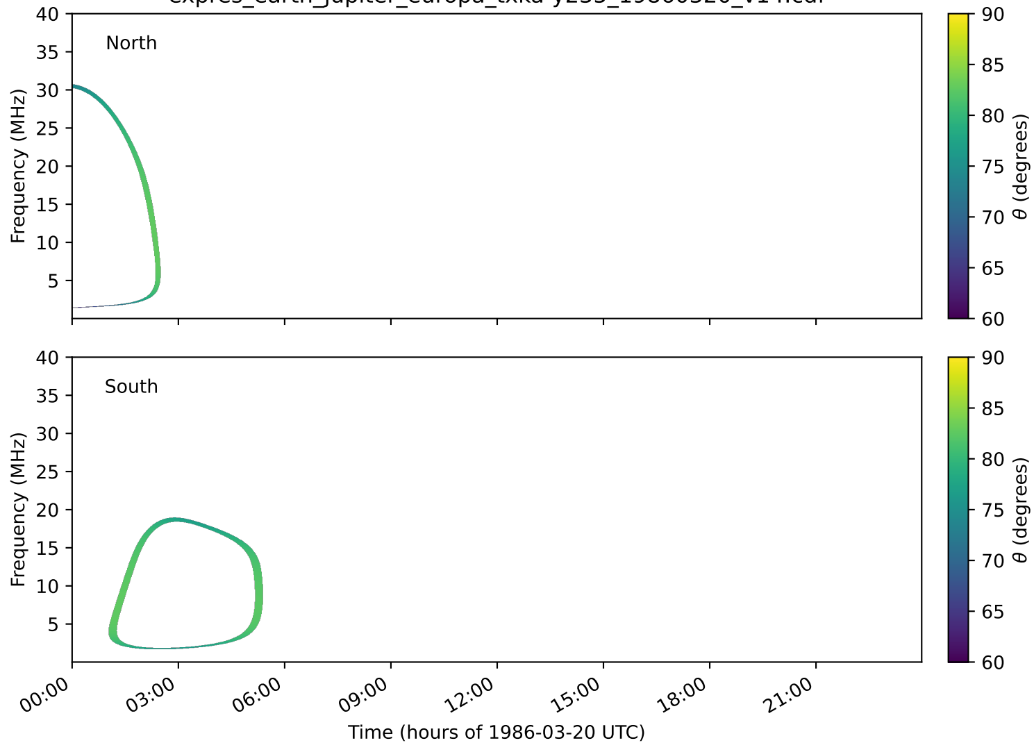
expres_earth_jupiter_europa_txka-y235_19860320_v14.cdf
