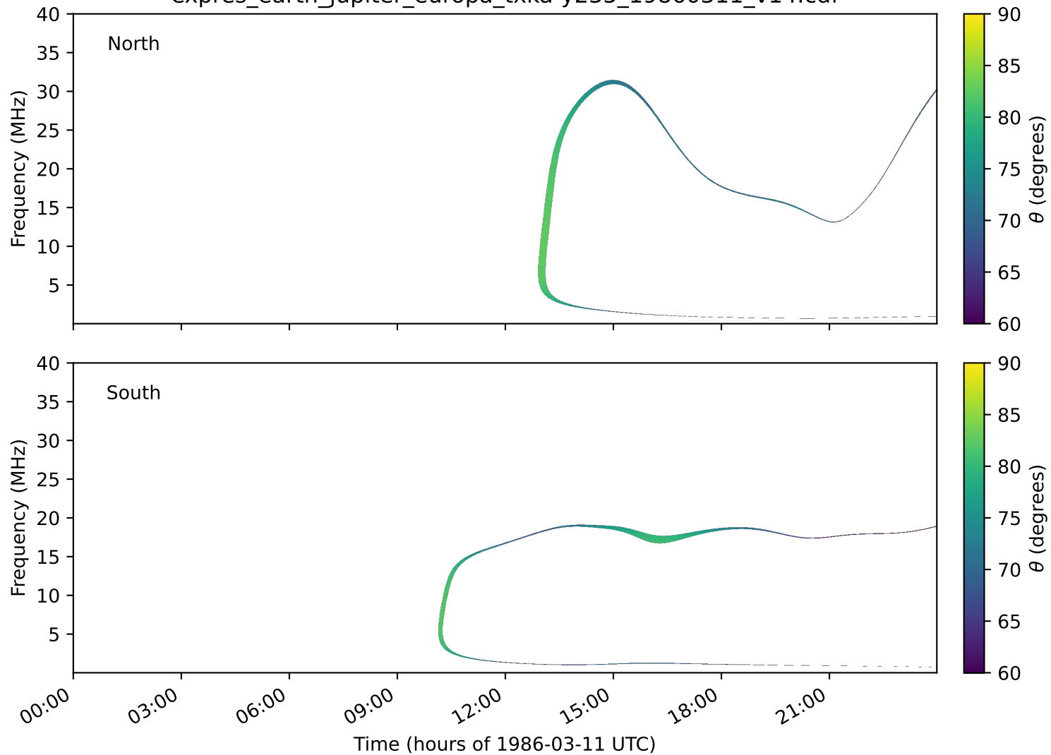
expres_earth_jupiter_europa_txka-y235_19860311_v14.cdf
