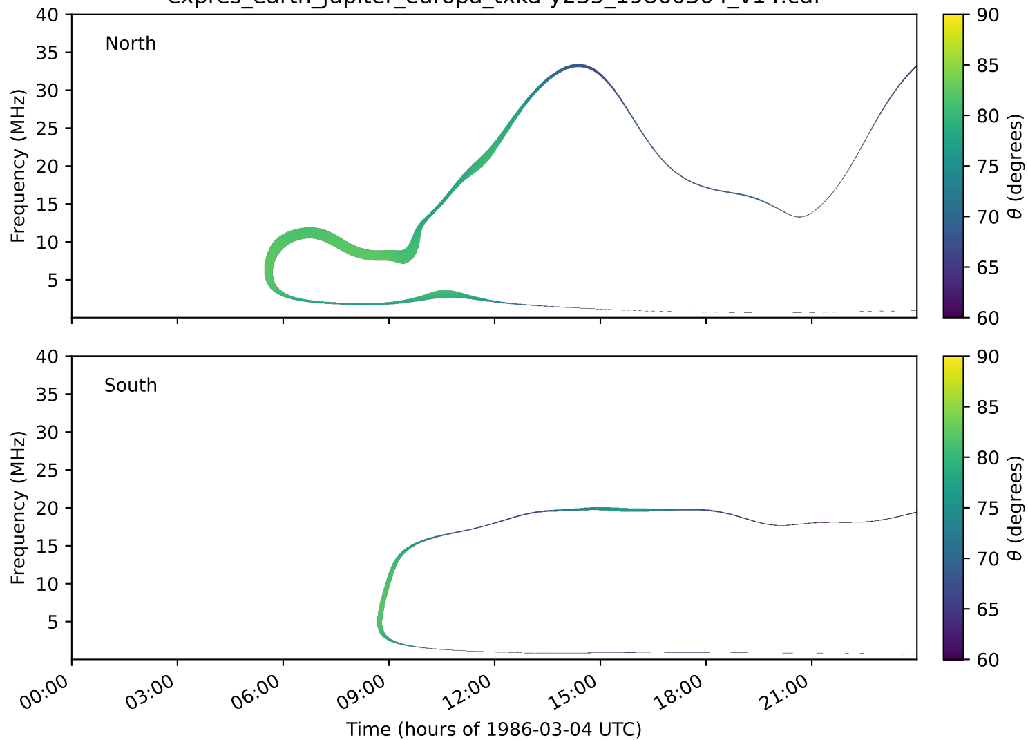
expres_earth_jupiter_europa_txka-y235_19860304_v14.cdf
