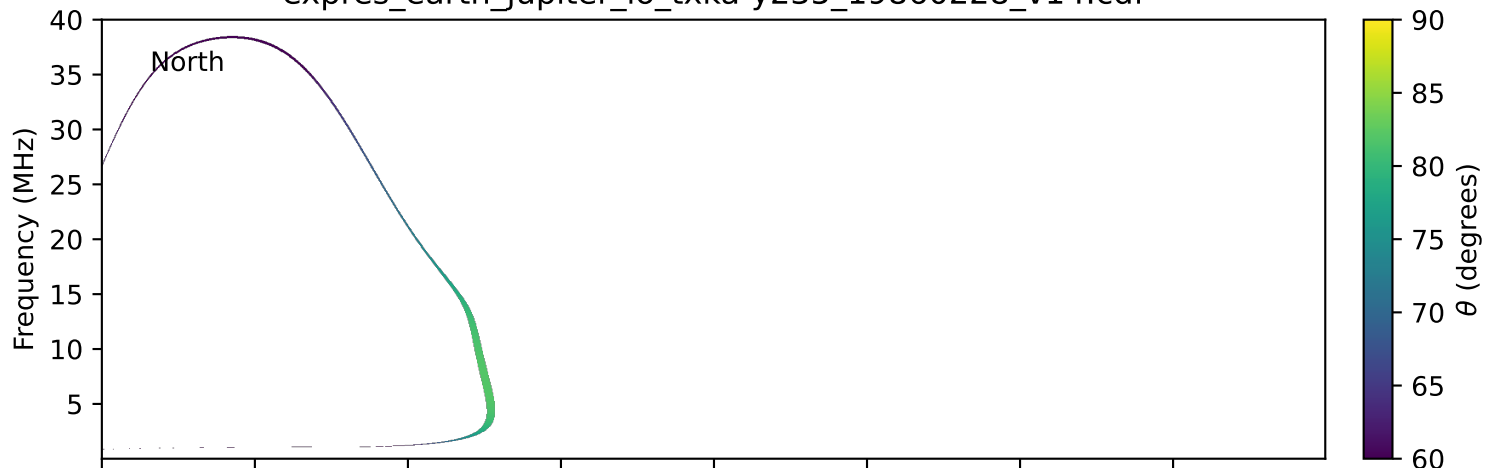
expres_earth_jupiter_io_txka-y235_19860228_v14.cdf
