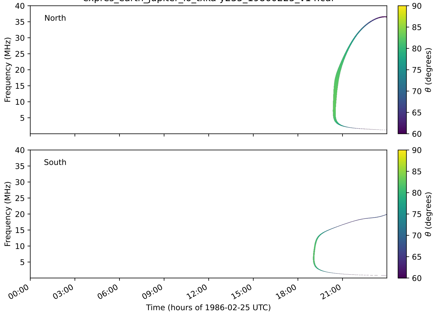
expres_earth_jupiter_io_txka-y235_19860225_v14.cdf
