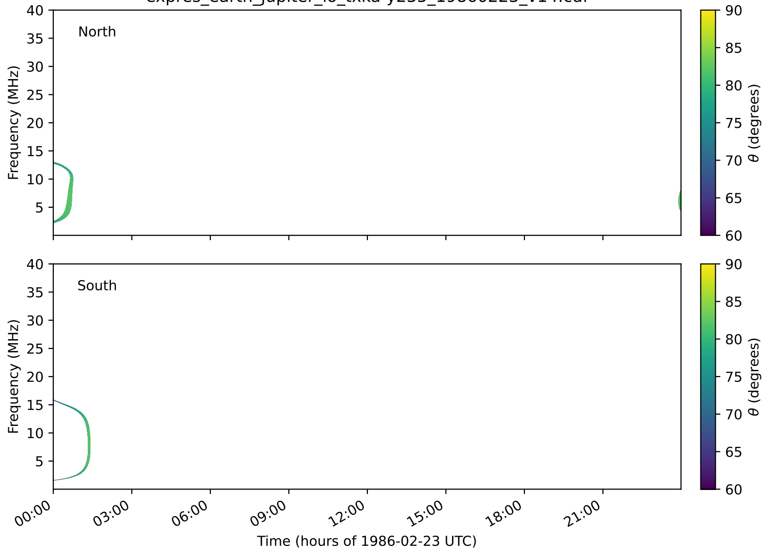
expres_earth_jupiter_io_txka-y235_19860223_v14.cdf
