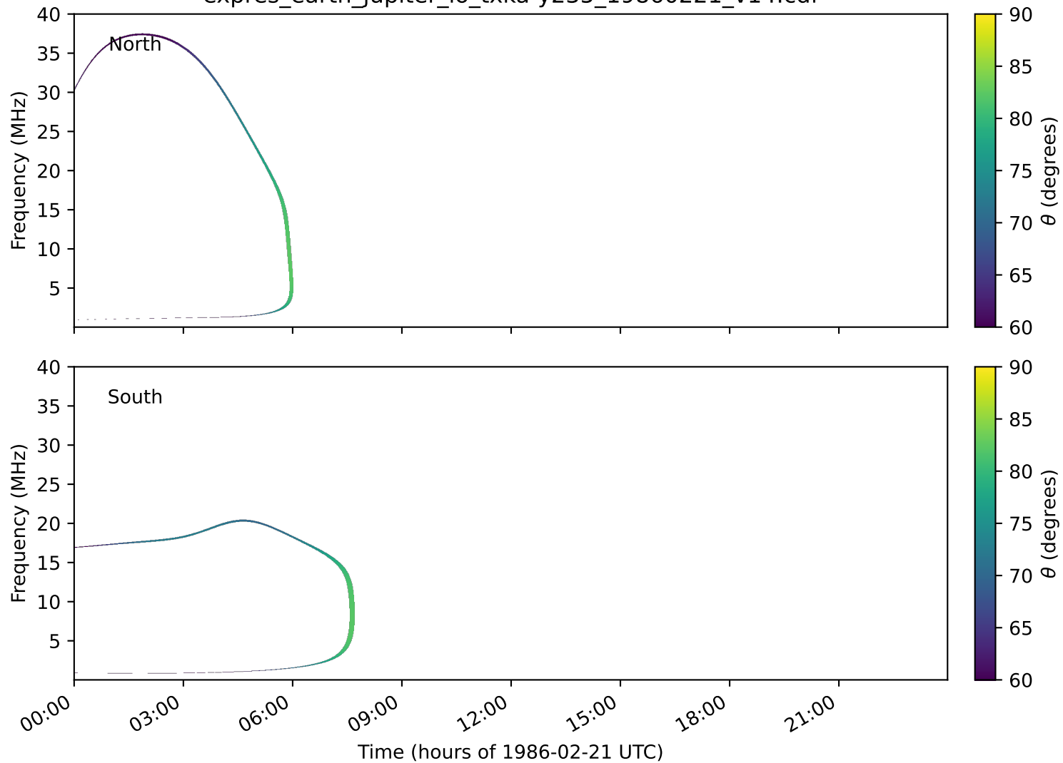
expres_earth_jupiter_io_txka-y235_19860221_v14.cdf
