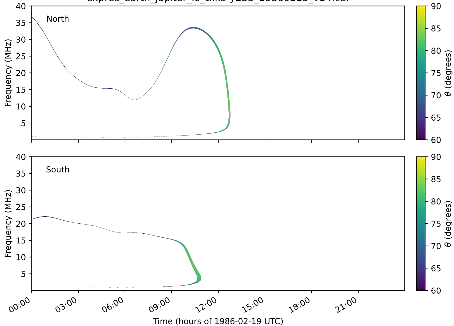
expres_earth_jupiter_io_txka-y235_19860219_v14.cdf
