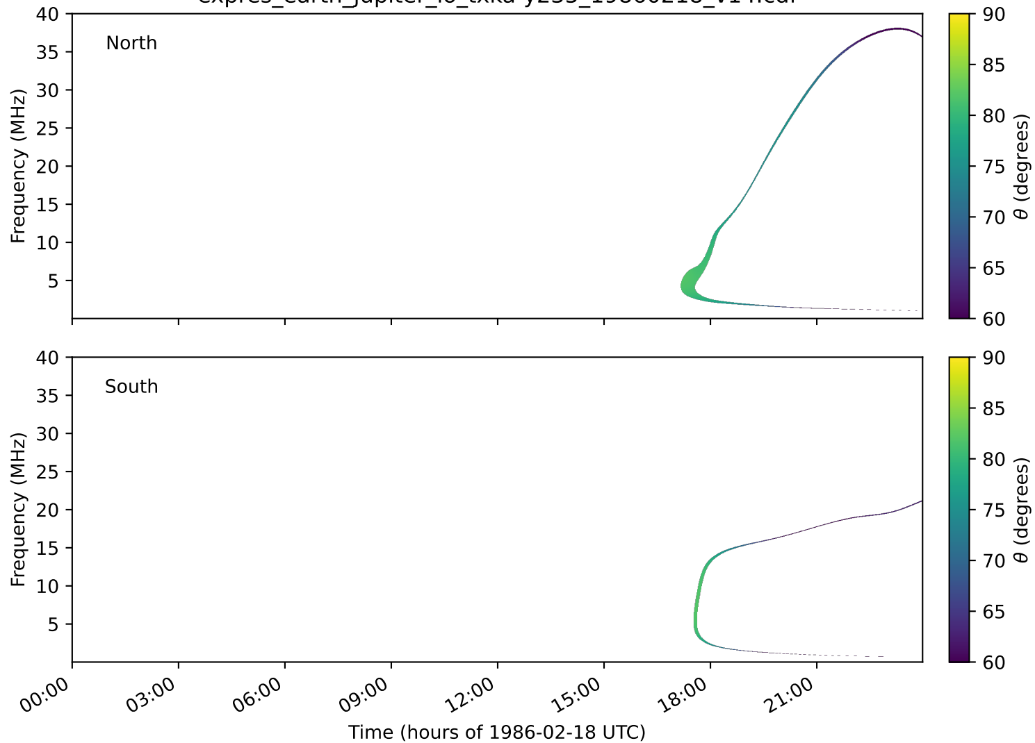
expres_earth_jupiter_io_txka-y235_19860218_v14.cdf
