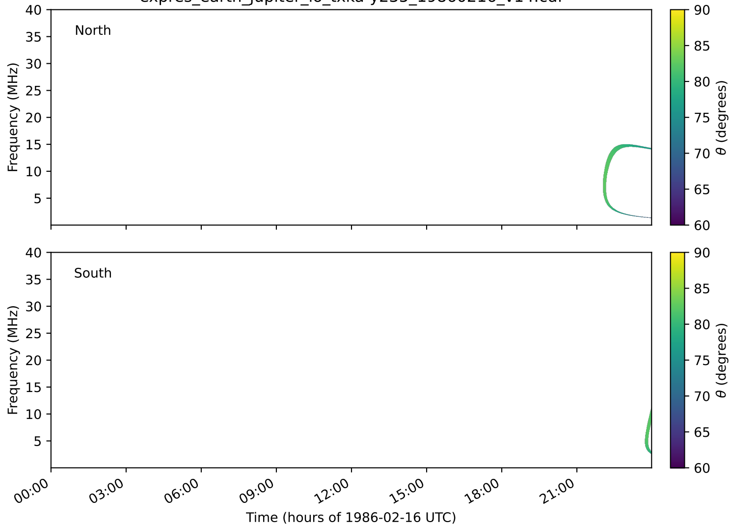
expres_earth_jupiter_io_txka-y235_19860216_v14.cdf
