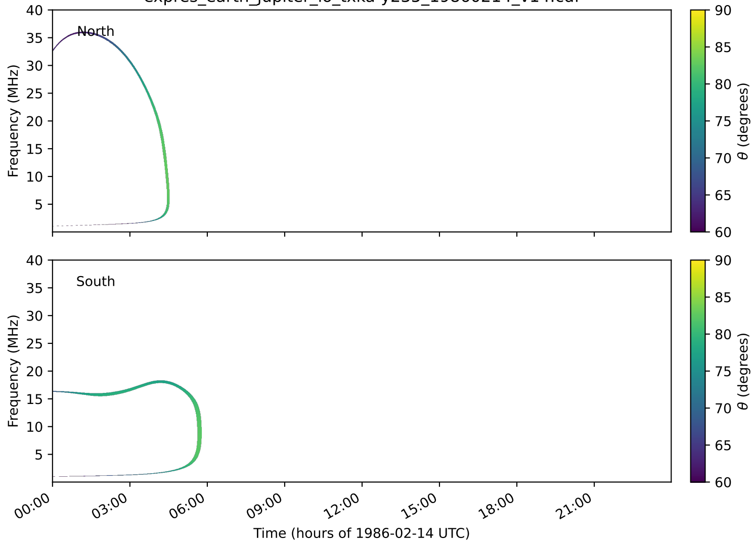
expres_earth_jupiter_io_txka-y235_19860214_v14.cdf
