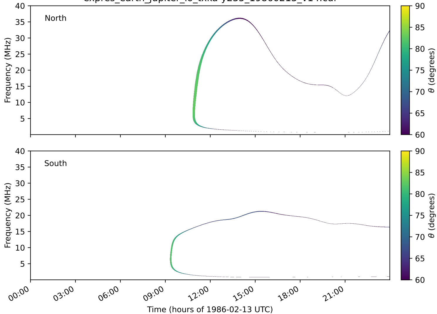
expres_earth_jupiter_io_txka-y235_19860213_v14.cdf
